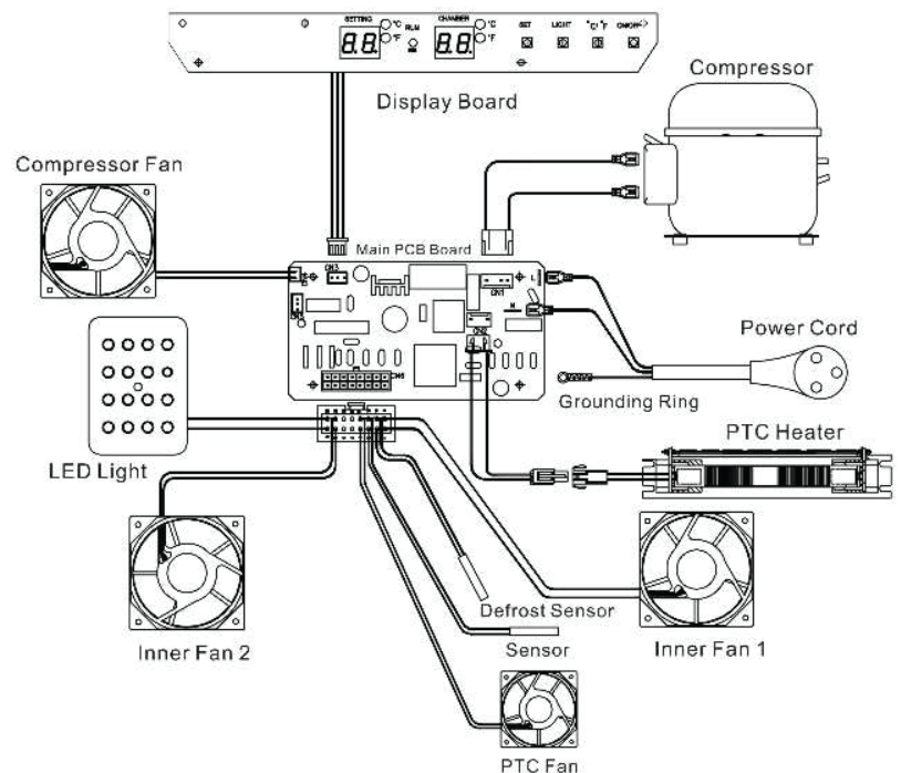
Electrical Diagram
