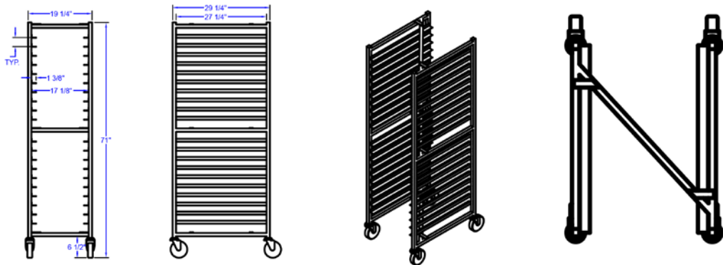
NESTED MOBILE PAN RACK- SQUARE TOP DESIGN
