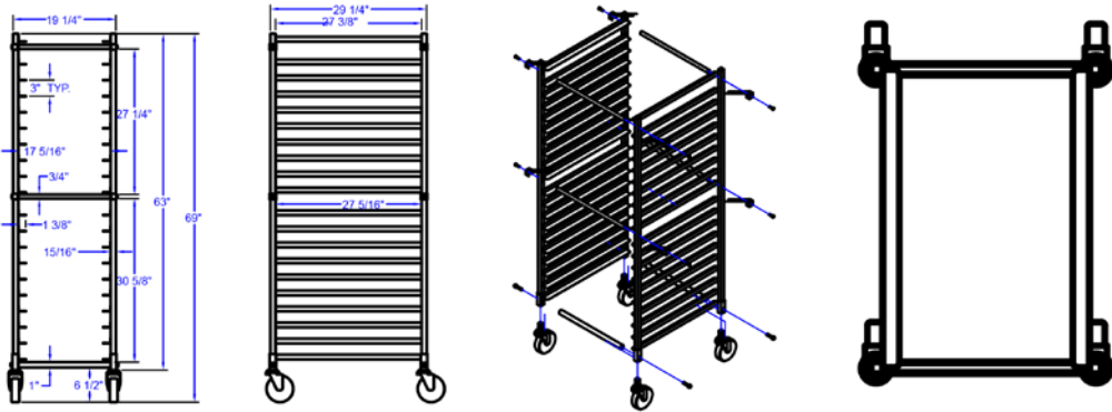
STANDARD MOBILE PAN RACK- SQUARE TOP DESIGN
