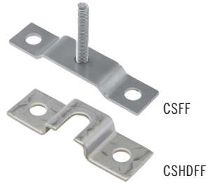
Hole diameter 9/16".
