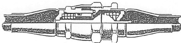
Figure 3 Coupling Halves Connected
