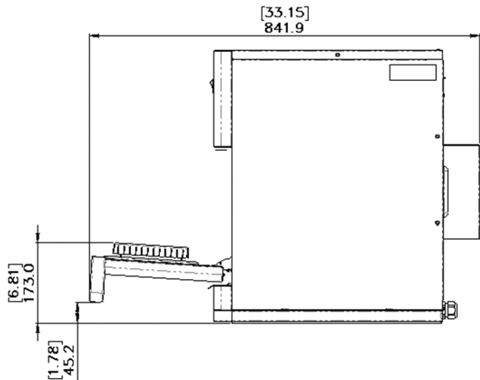
View from the right-hand side (door open)
