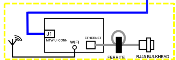
Module & Connections
