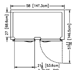
Plan - R/AHF232W
