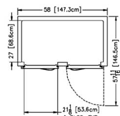
Plan - R/AHF232W
