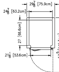
Plan - R/AHF132W
