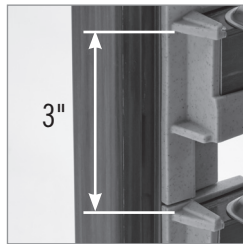
RAIL SPACING Wide 3" rail spacing offers greatest versatility and ease of use.
