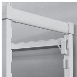
Traverse Dovetails
