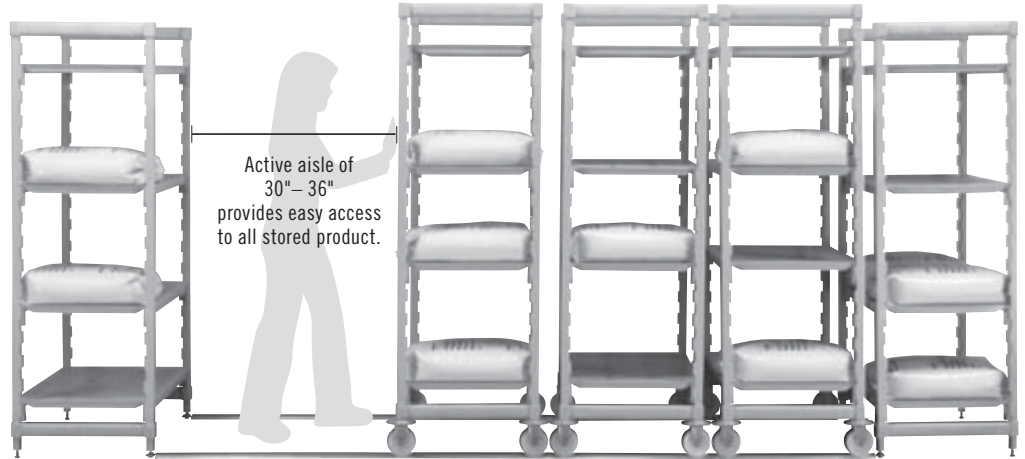
Stationary Unit
