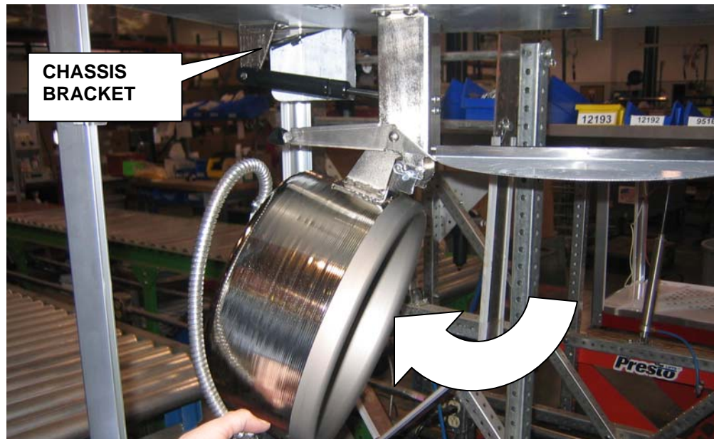
Figure 2: Swing kettle and attach gas spring.
