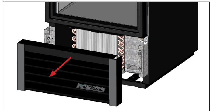
Fig. 3. Carefully remove the grill.
