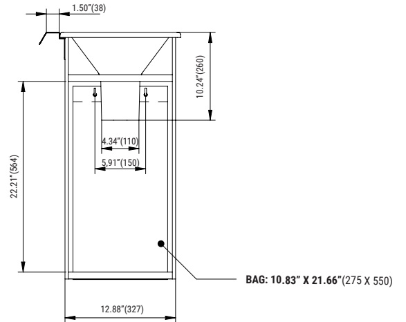
FRONTAL VIEW
