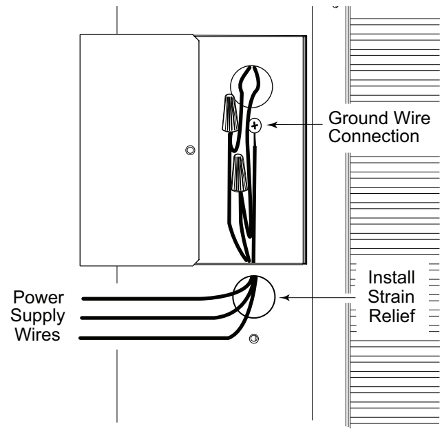
Electrical Connections, Back of Unit
