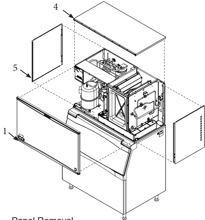
Panel Removal
