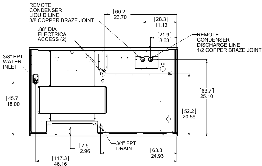
BACK VIEW
