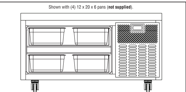
DRAWER PAN CONFIGURATION
