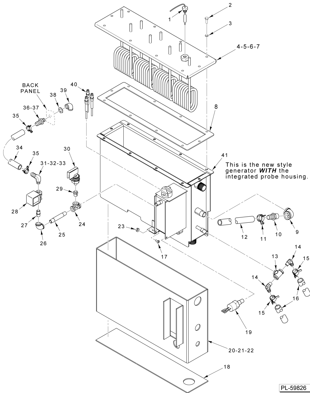
GENERATOR ASSEMBLY (S/N 463003747 THRU S/N 463023094)
