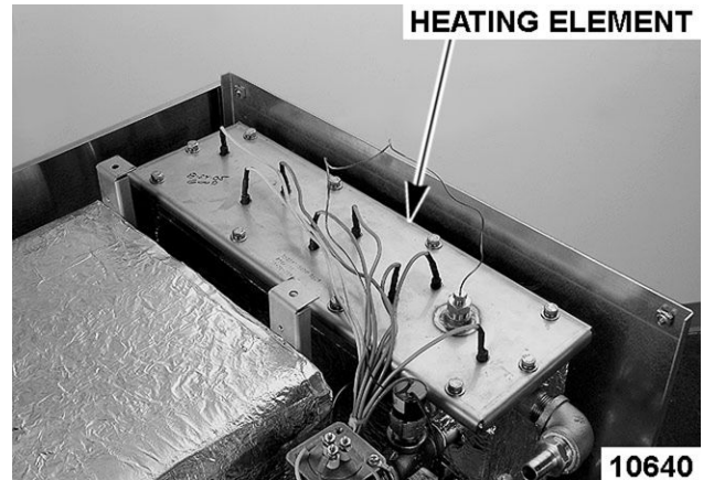
HEATING ELEMENT 10640 Fig. 41
