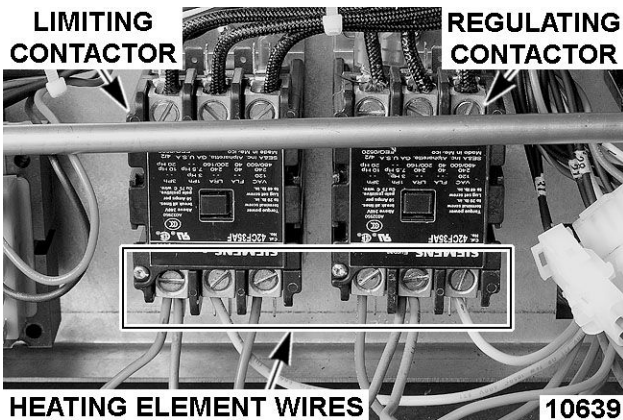
LIMITING CONTACTOR REGULATING CONTACTOR HEATING ELEMENT WIRES 10639 BASIC MODEL SHOWN
