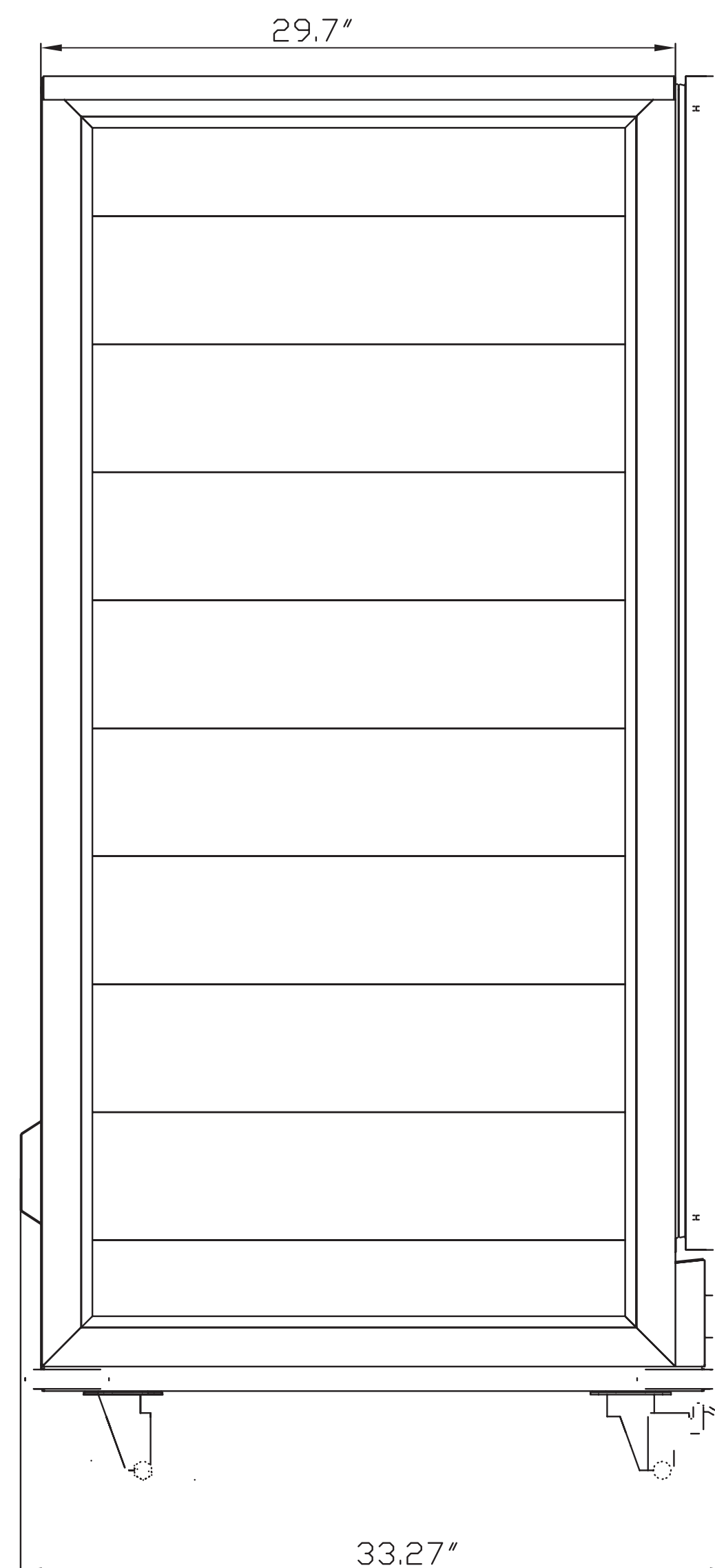
Side View
