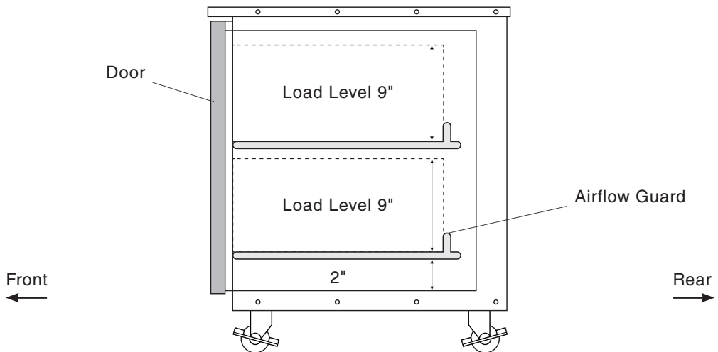
Side View
