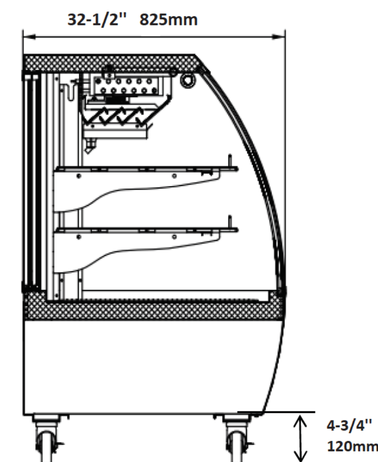
Side View
