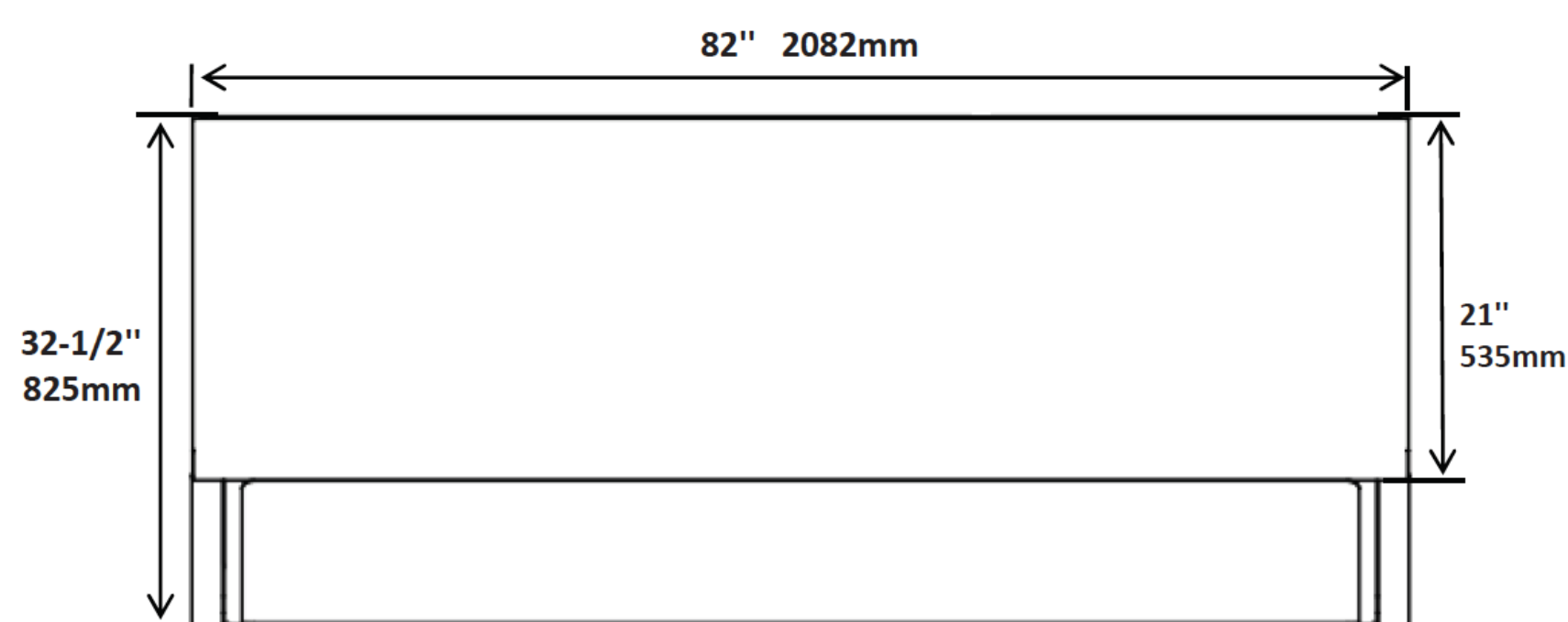
Top View
