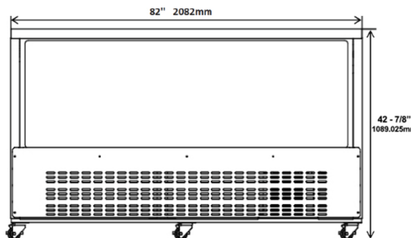
Front View
