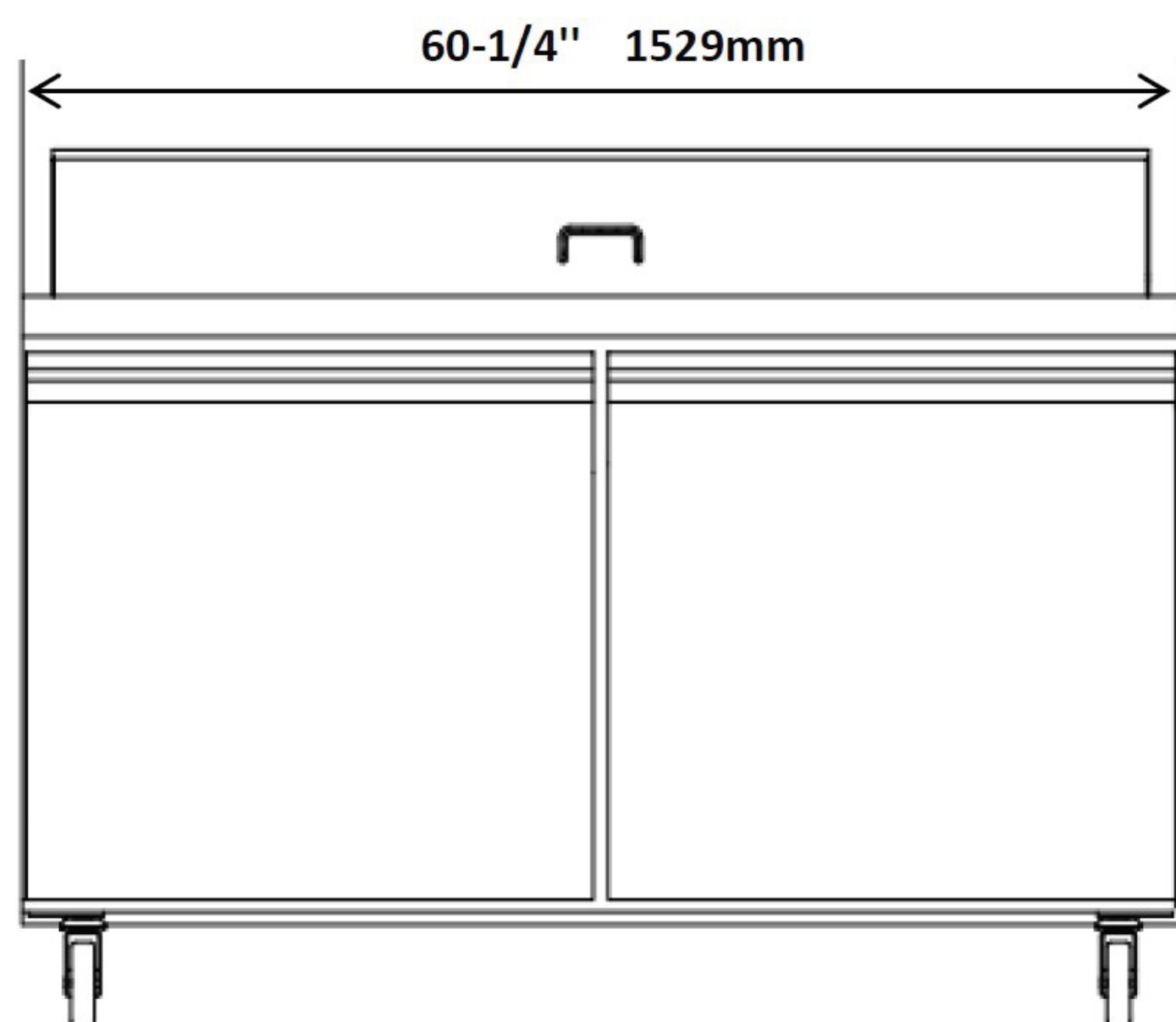
Front View
