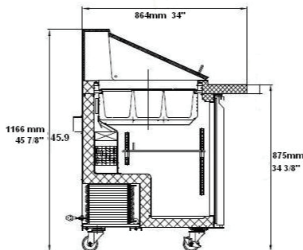
Side View
