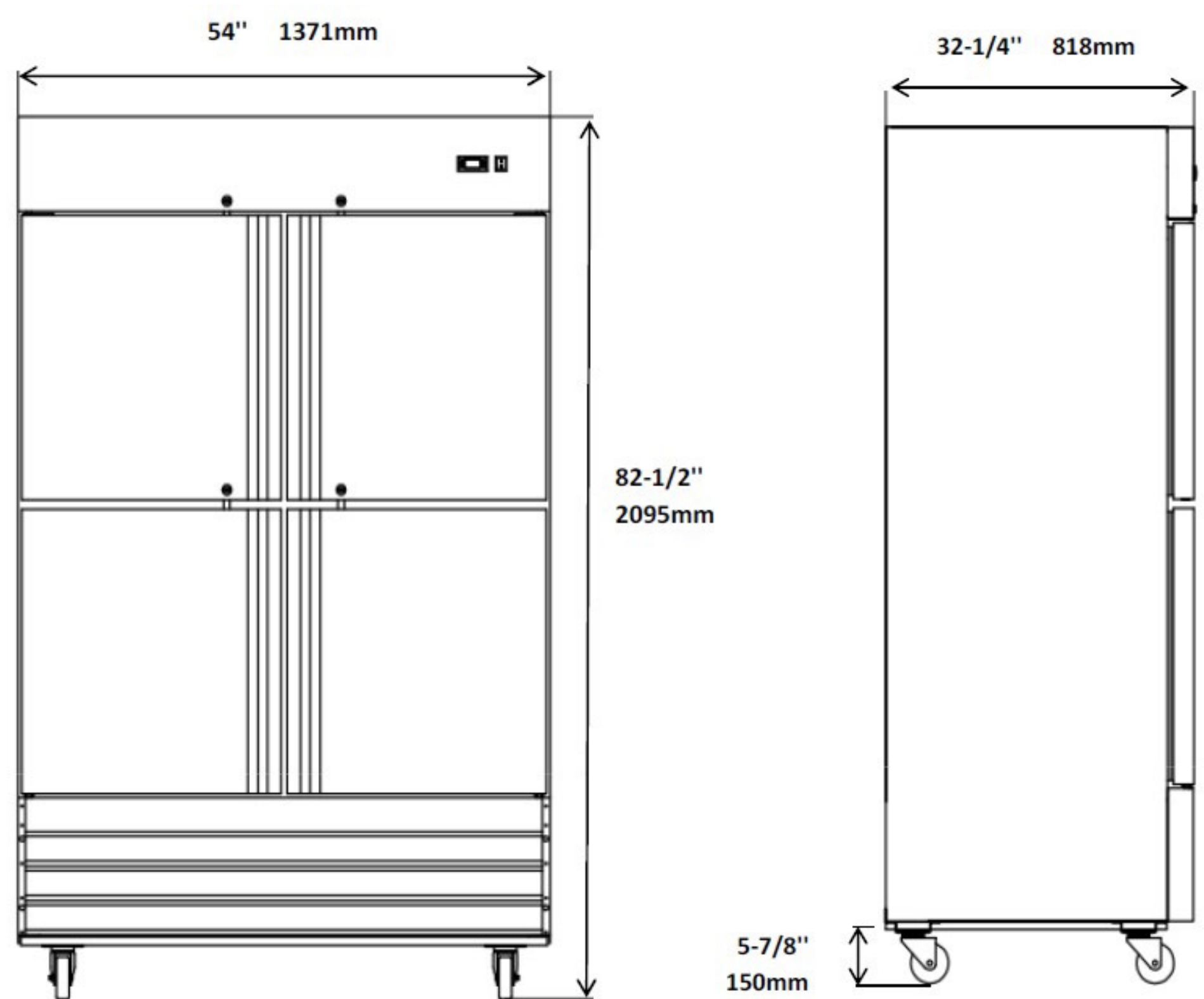
Front View
