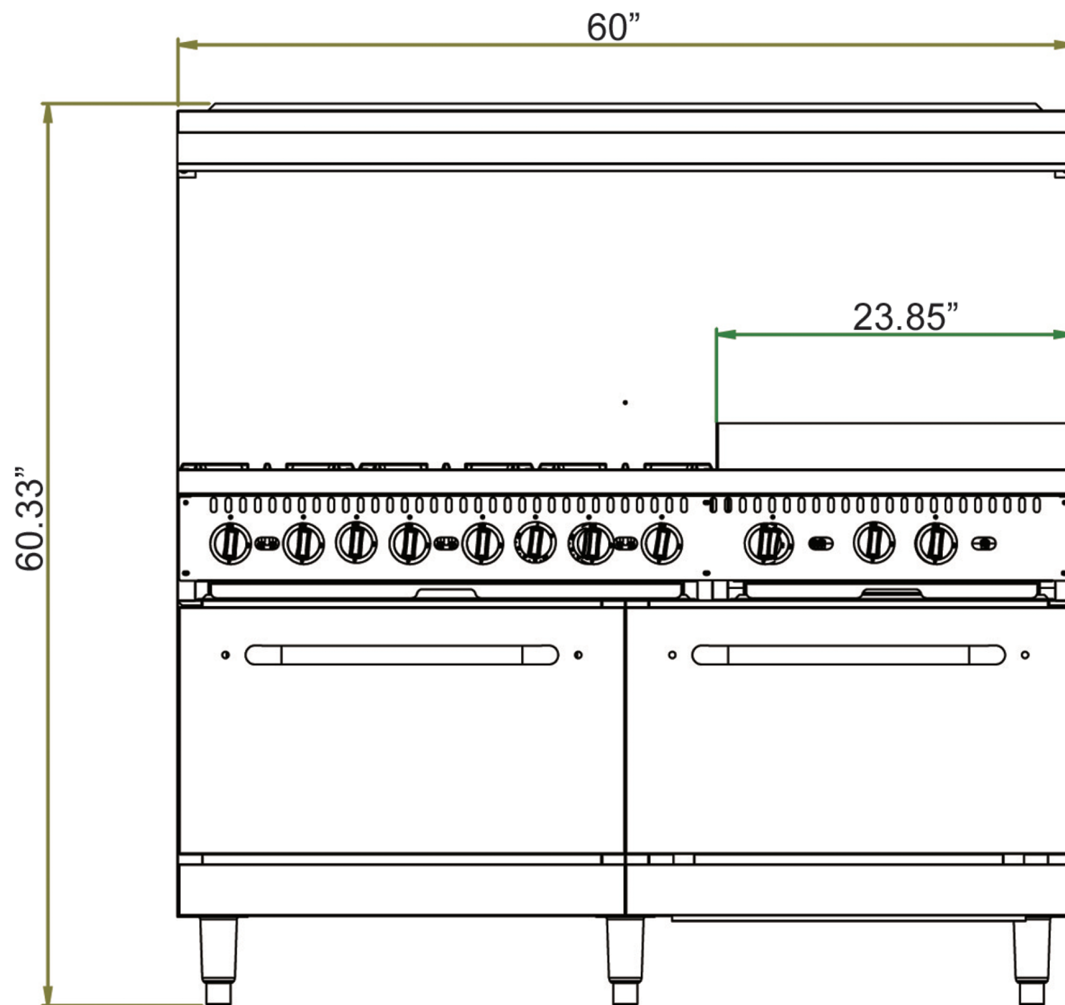
Front View
