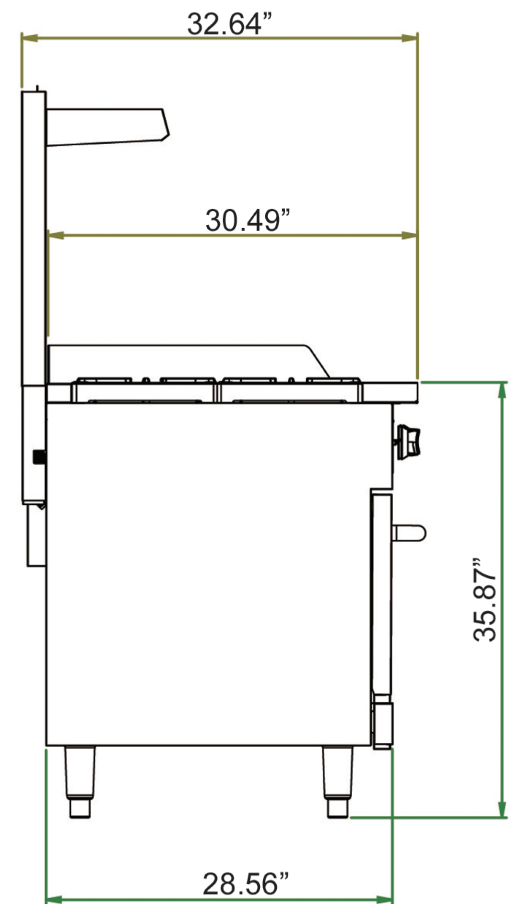
Side View
