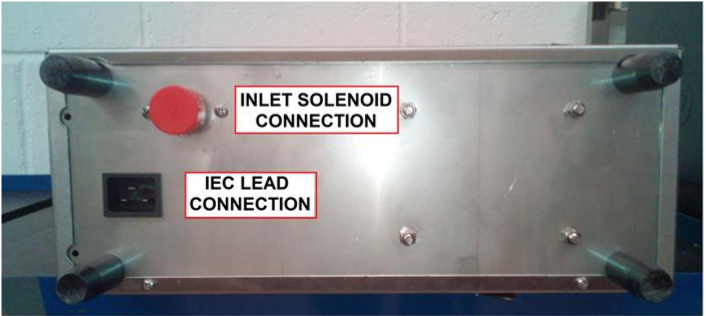
Figure 8 - Base of SP9 Undercounter Unit
