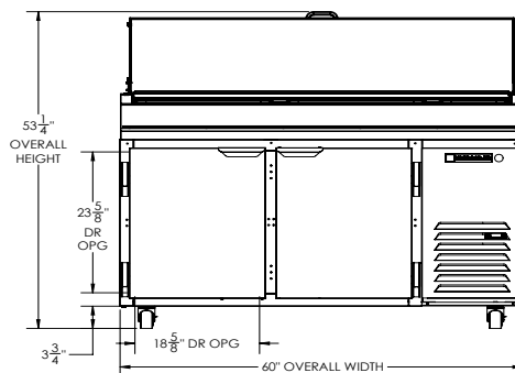
ELEVATION VIEW
