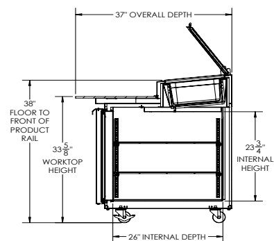
ELEVATION VIEW
