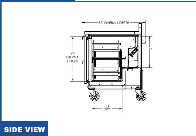
ELEVATION VIEW
