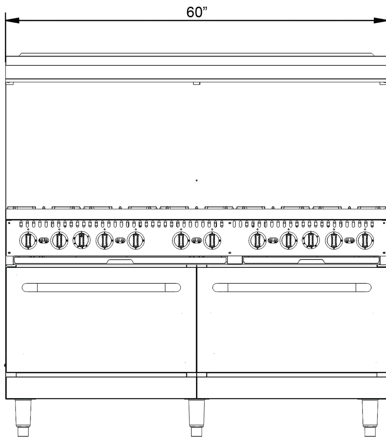
Front View
