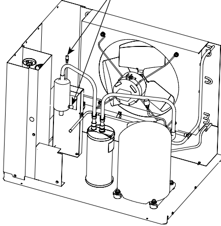
ALTERNATE CONNECTIONS AT CONDENSING UNIT SCHRADER VALVES
