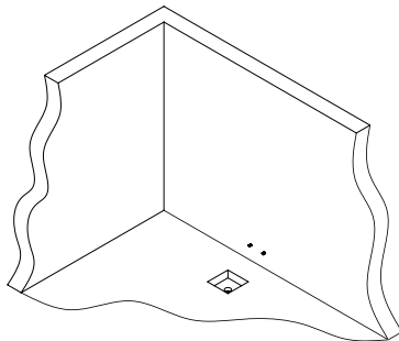
Suggested Plumbing Rough-In (Open Floor Drain) *** SEE DETAIL (A) ***
